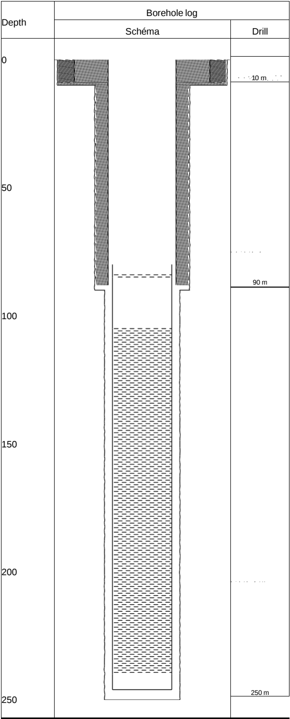
Drawing No. 1 Tentative Log for Borehole
